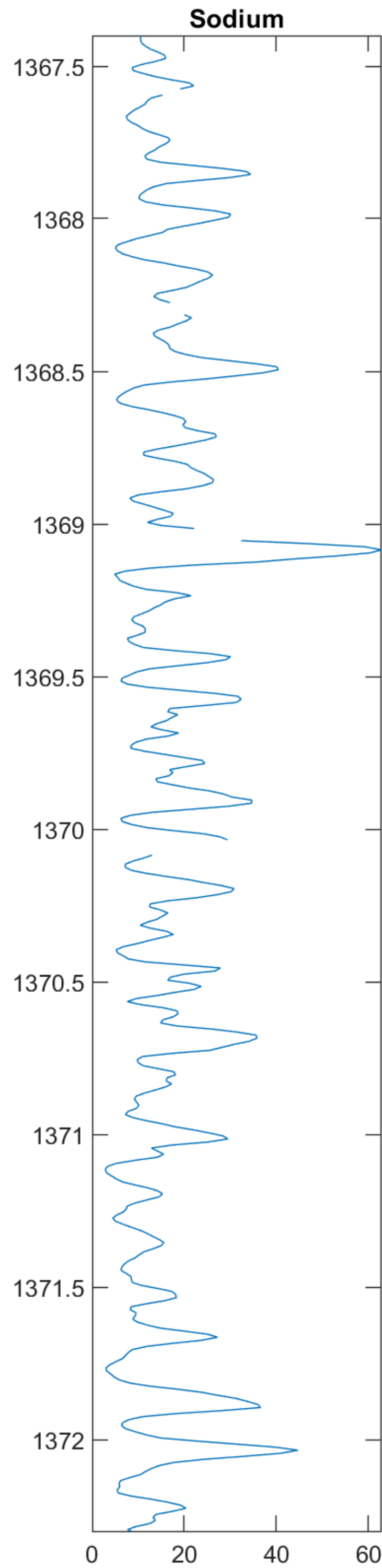
Graph 3: Sodium - at a Depth of ~1300m
