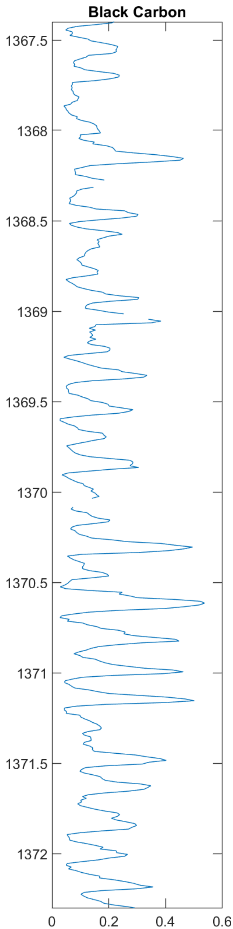
Graph 4: Black Carbon - at a Depth of ~1300m
