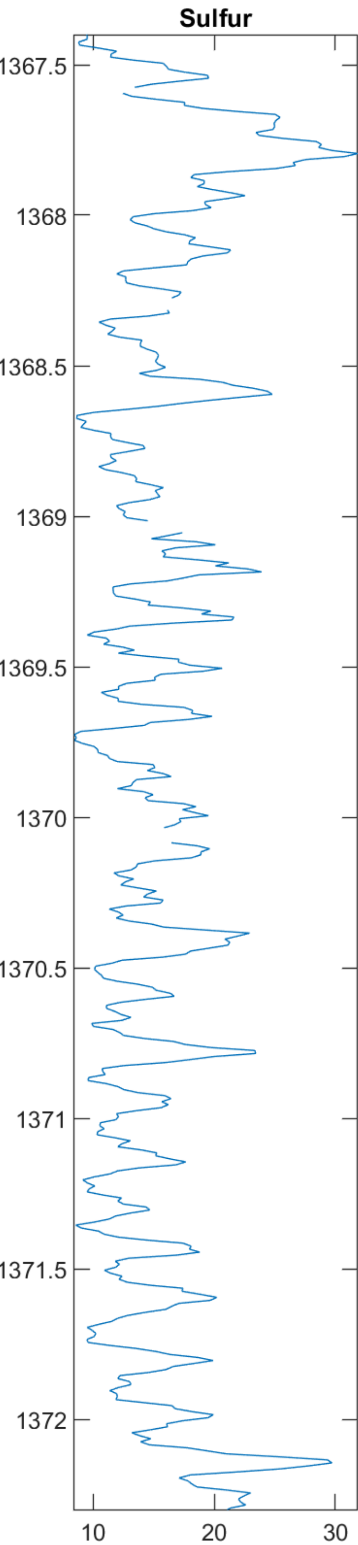
Graph 2: Sulfur - at a Depth of ~1300m
